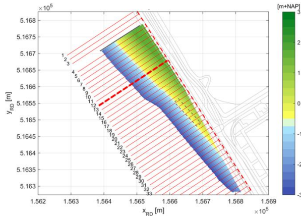
Figure 9 Overview of measurement trajectories used for the morphological recordings with cross-shore profile no 12 indicated by the red dotted line.
