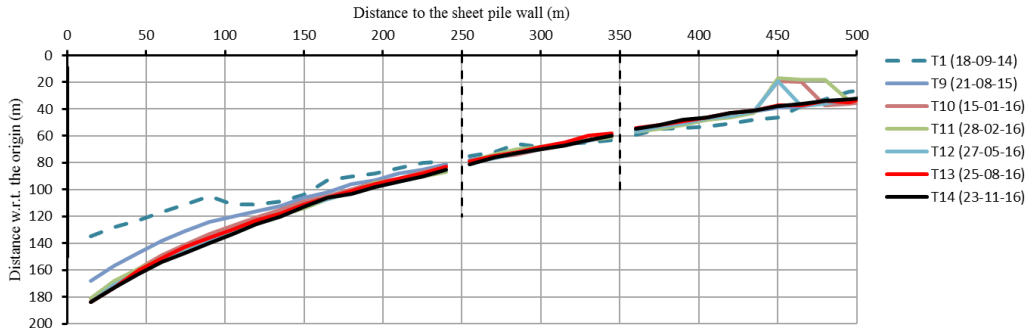
Figure 15 Development of the longshore position of the contour representing the lower zone.
