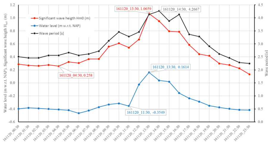
Figure 5 Overview of observed conditions during the autumn storm of November 20, 2016 showing the development of the water level (blue line), the wave height (red line) and the wave period (black line).
