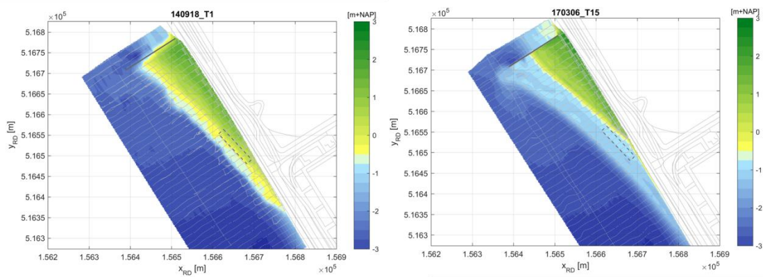
Figure 7a Development of the bathymetry with the levels at the start of the monitoring programme on September 18, 2014; Figure 7b The result of the most recent measurement on March 6, 2017.
