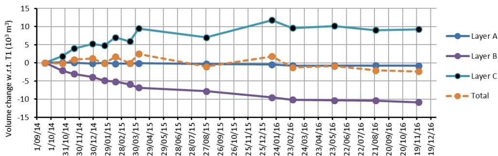
Figure 13 Development of the volume in the distinguished vertical zones with respect to the initial volume (T1).
