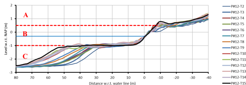
Figure 12 Development of the cross-shore profile shape at location 12, plotted relative to the intersection with the NAP-0.3 m level. Including the definition of the upper (A), middle (B) and lower layer (C).
