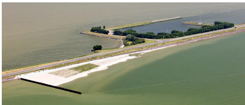
Figure 3 Overview of pilot section direct in June 2016 (two years after construction) showing the adjusted contour as well as the well-developed vegetation in specific plots of the test section (photo: Jurriaan Brobbel).
