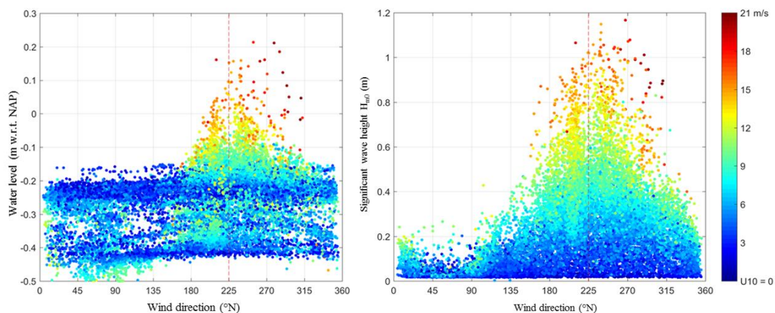
Figure 4a Relation between the water level and wind direction; Figure 4b Relation between the significant wave height and wind direction on the right-hand side, including colours indication the wind velocity. The vertical dashed lines refer to the cross-shore orientation of the pilot section at 225° N.
