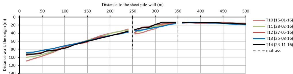
Figure 14 Development of the longshore position of the contour representing the middle zone.
