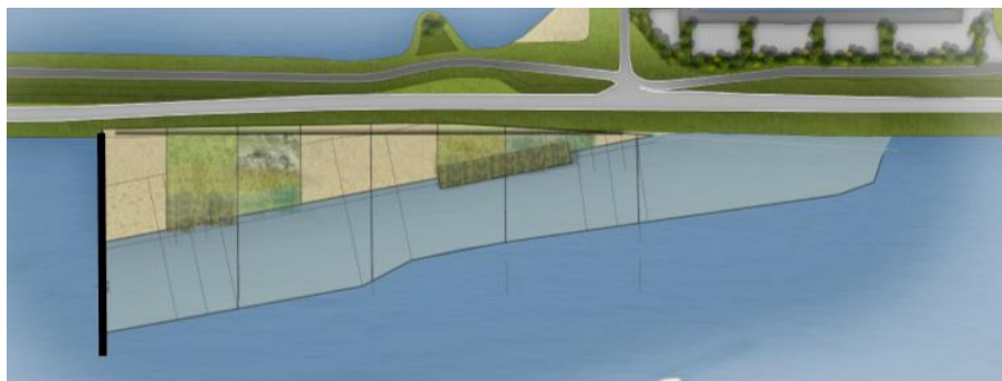
Figure 2 Lay-out of the pilot section with four sections of each 100 m width and each section planted manually, while the other half is left to develop on its own. The willow faggots matras is positioned in the right-hand smaller section.
