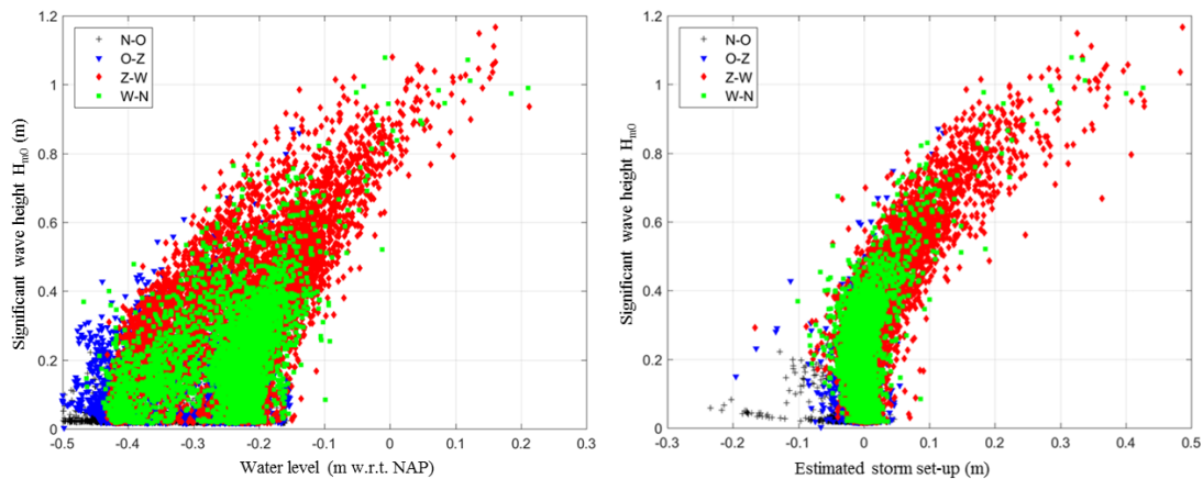
Figure 11a Overview of all combinations of water level and wave heights; Figure 11b Overview of all combinations of the estimated storm set-up and wave heights all for four sections of wind direction.
